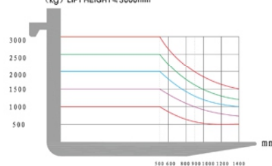
Load Chart (kg) LIFT HEIGHT ≤ 3000mm
